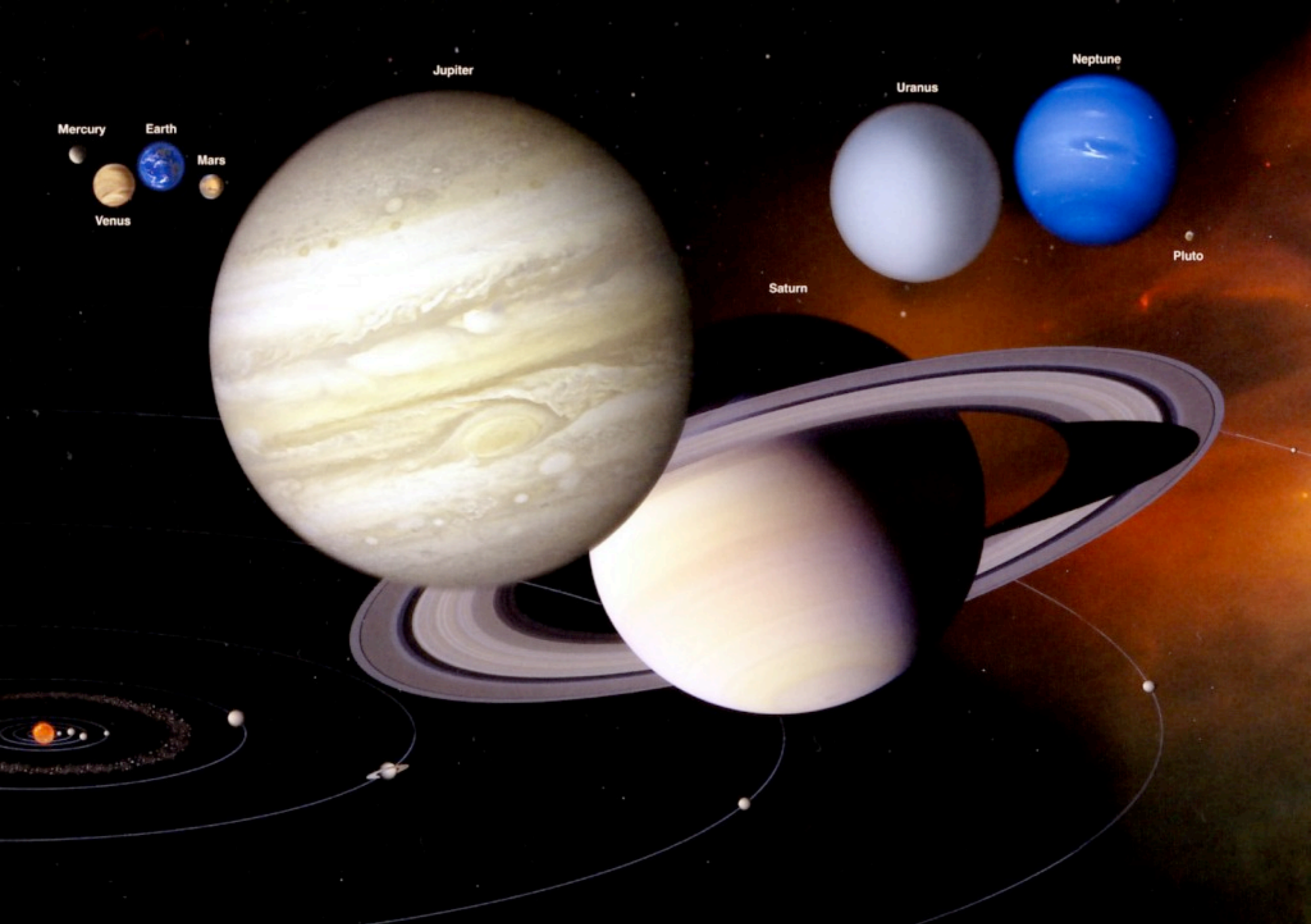
Relative sizes of the planets (including the dwarf planet Pluto)
